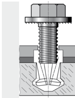
Undercut anchor bore
