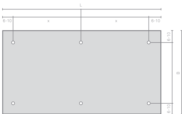
Multiple field plate | 2 rows horizontal
