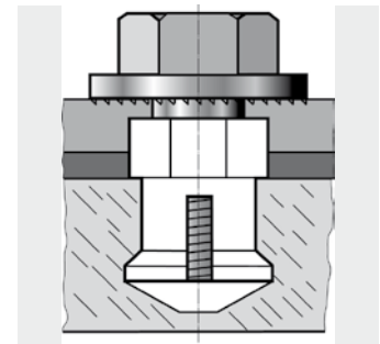
Undercut anchor bore
