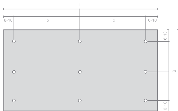
Multiple field plate | 3 rows horizontal
