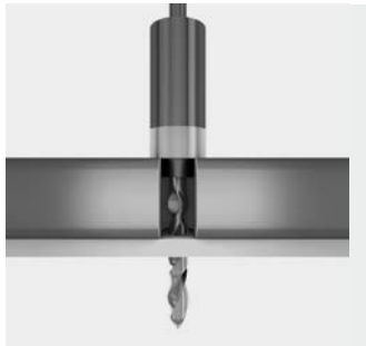
Drilling with drilling jig
