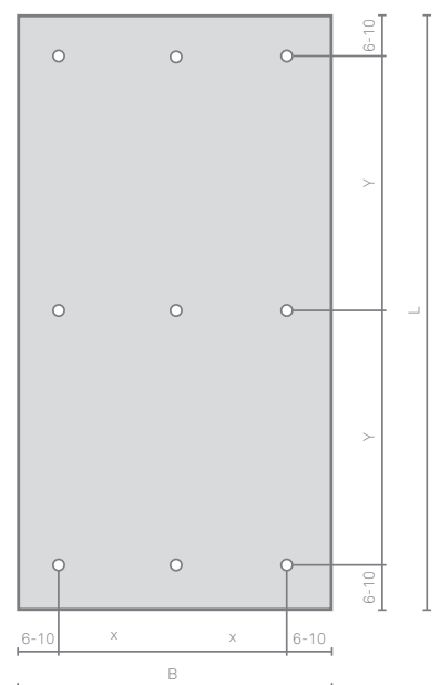
Multiple field plate | 3 rows vertical
